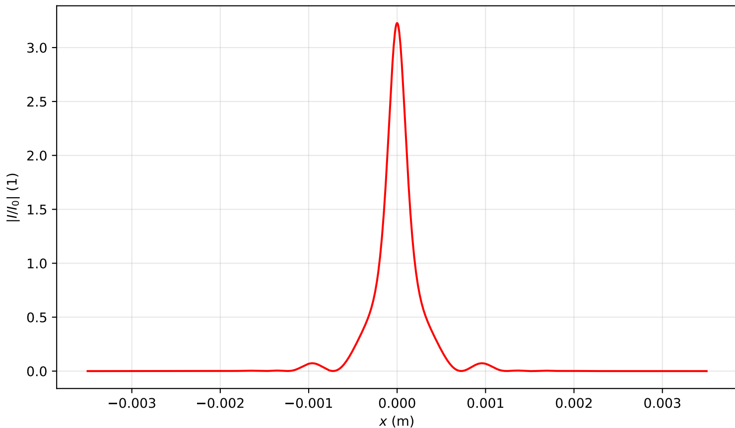
Intensity profile I(x, y = 0, z = 1.433)/I_0 , P_{in}=3.0P_{cr} , artificial time
